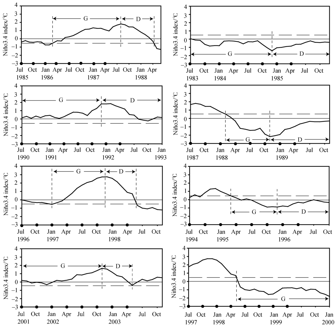
Figure 1 Observed Niño3.4 index of four El Niño events (left column) and La Niña events (right column) between 1982–2007. “G” represents growth phase, and “D” denotes the decay phase. The dots located on the horizontal axis signify the initial times of the predictions.
